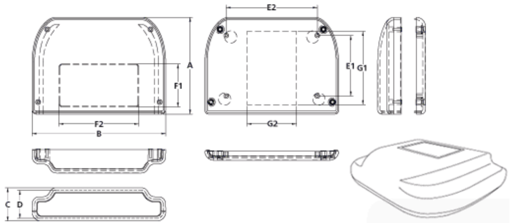
AG-54 with display window
